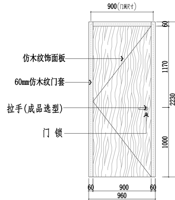
M0922
