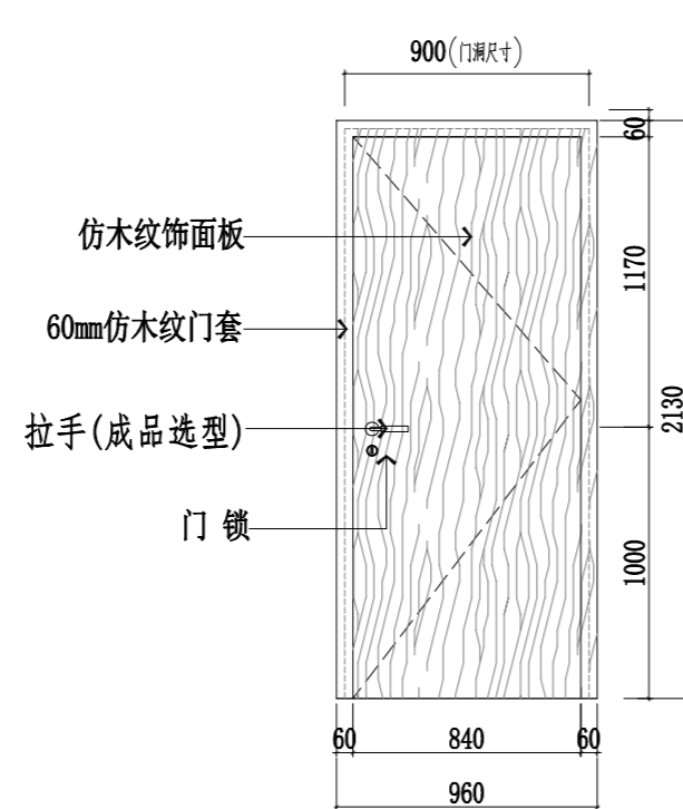
M0921
