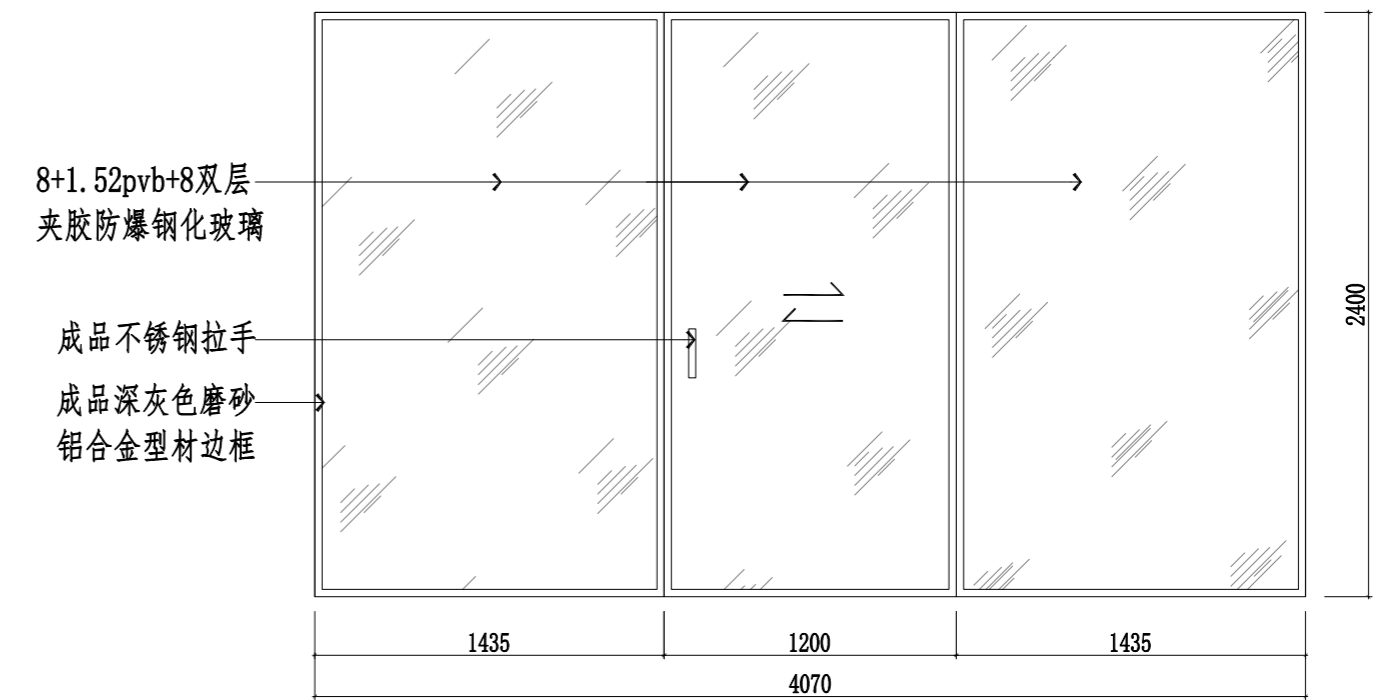
LM1222
