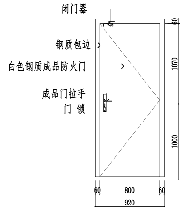
FM乙0921
