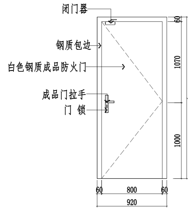
FM甲0921
